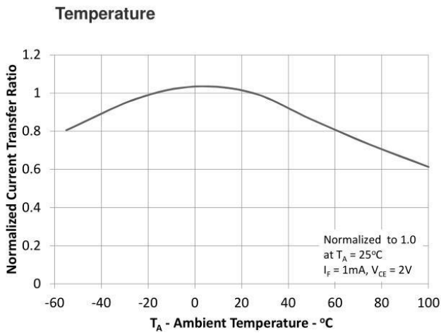
Figure 7. Normalized Current Transfer Ratio vs. Ambient
