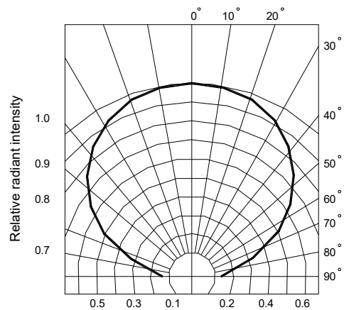
Fig.6 Radiation diagram
