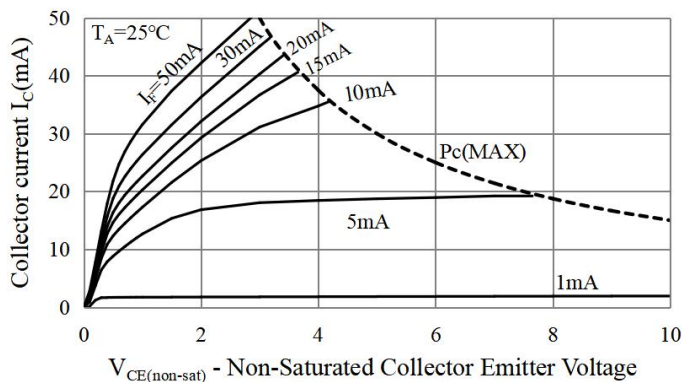
fig.5 Collector Current vs. Non-Saturated Collector Emitter Voltage
