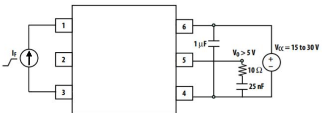
Figure 19: I FLH Test Circuit
