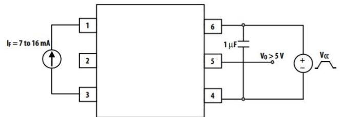
Figure 20: UVLO Test Circuit
