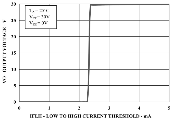
Figure 7: Transfer Characteristics
