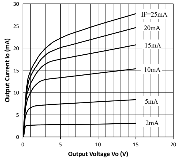
OUTPUT CURRENT vs. OUTPUT VOLTAGE
