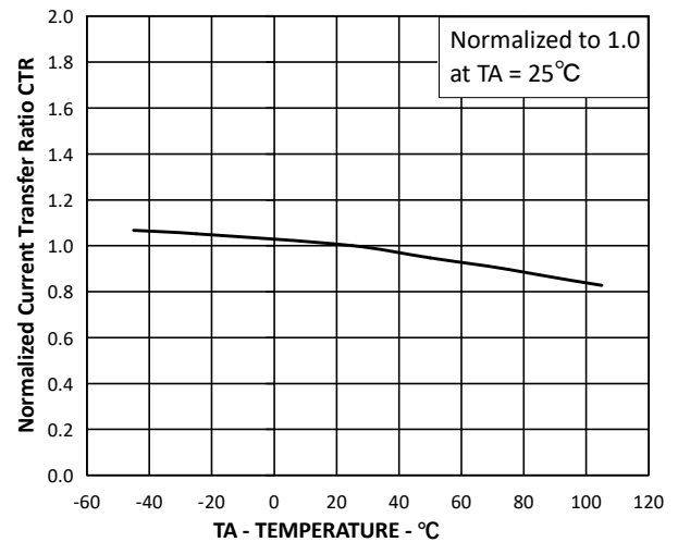
CURRENT TRANSFER RATIO vs. TEMPERATURE
