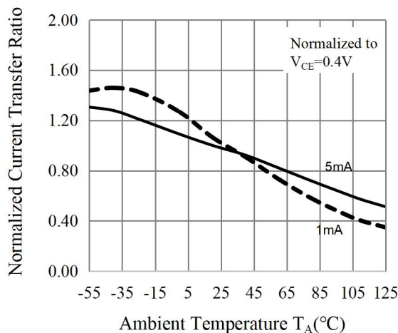
Fig.8 Relative Current Transfer Ratio vs. Ambient Temperature
