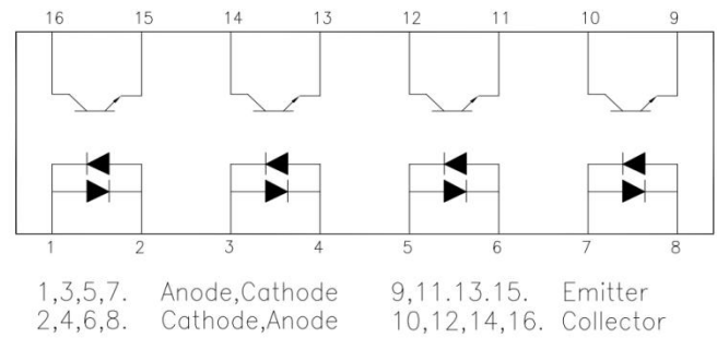
PIN NO. AND INTERNAL CONNECTION DIAGRAM
