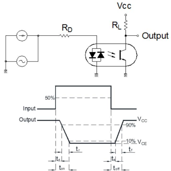
Fig.14 Switching Time Test Circuit & Waveforms
